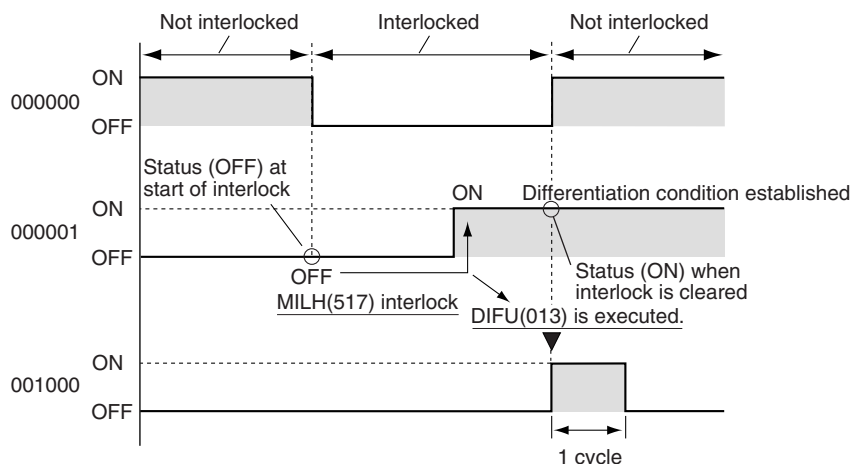
Timing Chart
