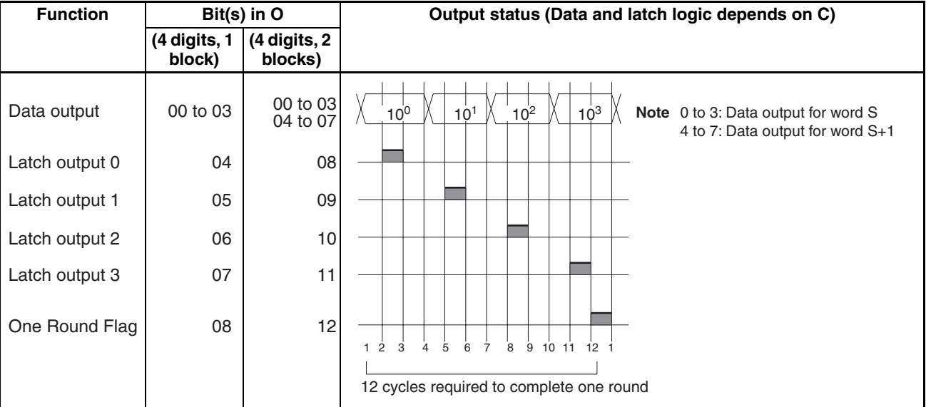
Timing Chart
