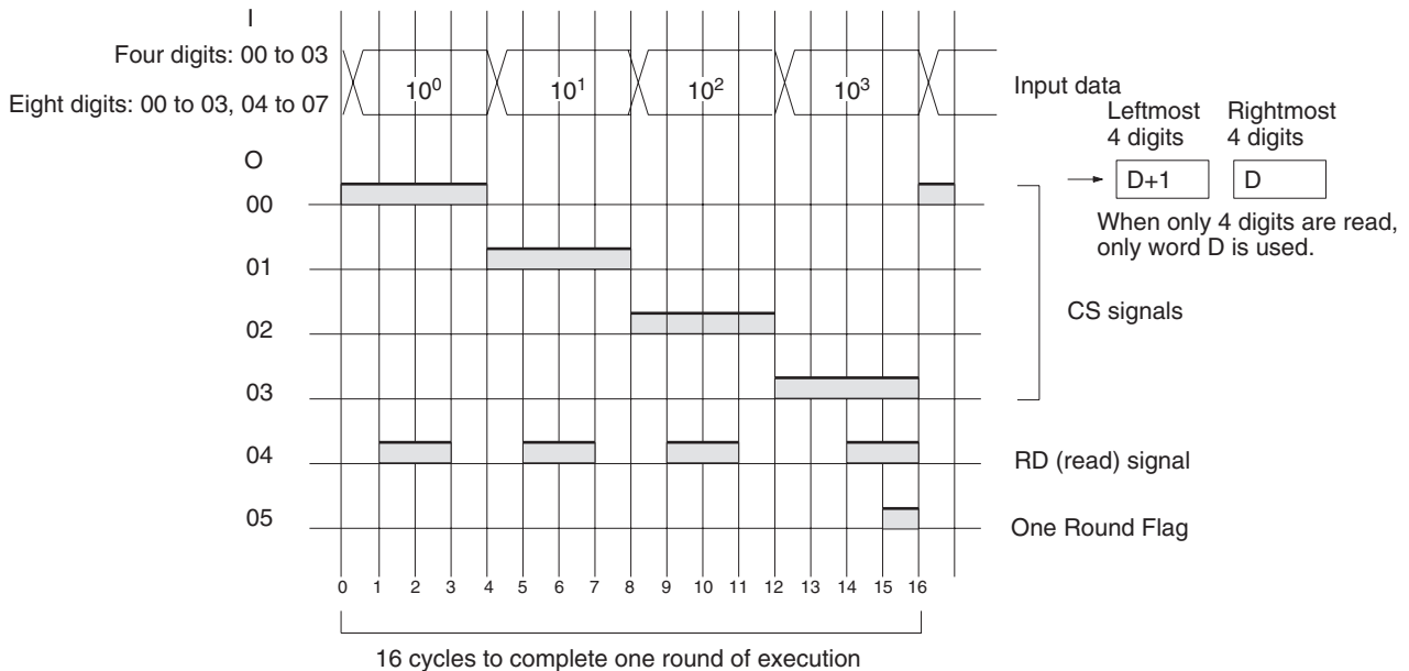
Timing Chart
