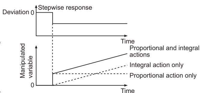
Manipulated Variable for Integral and Proportional Actions Together
